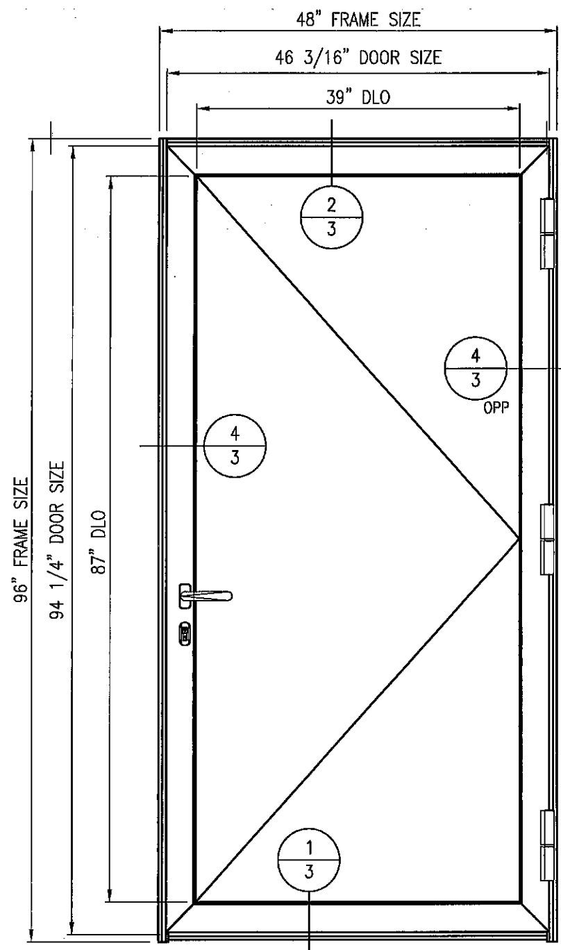
ELEV SERIES 4000 TERRACE DOOR STANDARD (OUT SWING) Scale: 3/4" = 1'-0"
