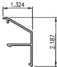
5 SUN-4115 SILL SCREW COVER Scale: 6" = 1'-0"
