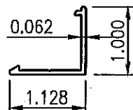
4 SUN-4114 HEAD/JAMB SCREW COVER Scale: 6" = 1'-0"
