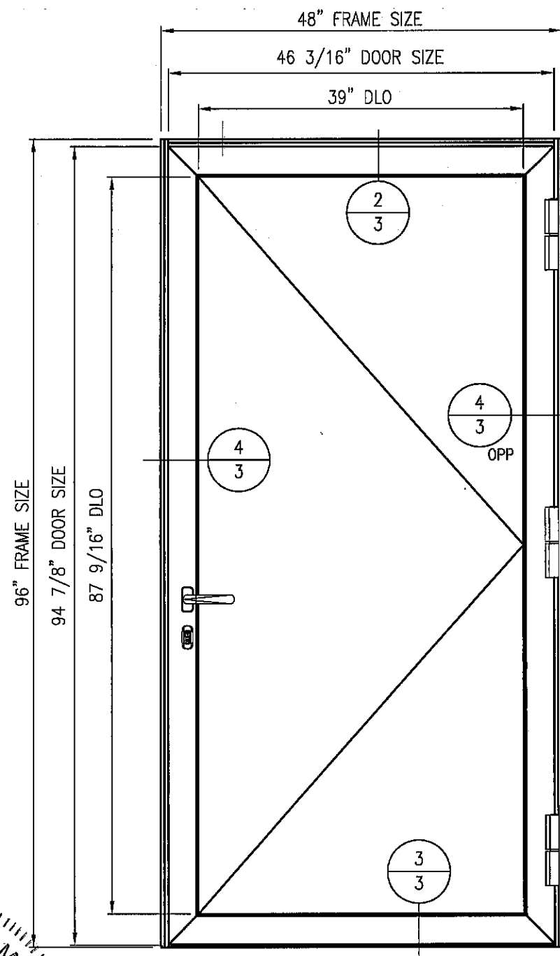
ELEV SERIES 4000 TERRACE DOOR ADA (OUT SWING) Scale: 3/4" = 1'-0"
