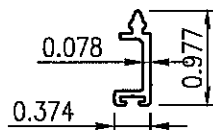
7 SUN-4120 ADA DOOR EXTENSION Scale: 6" = 1'-0"
